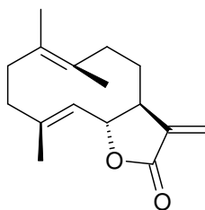
costunolide
