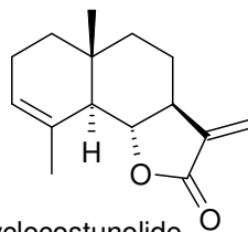
cyclocostunolide
