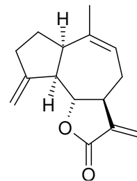
eremanthine
