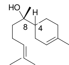
(-)-alpha-bisabolol [4S,8S]
