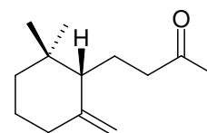
dihydro-gamma-ionone
