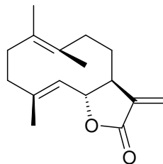
costunolide
