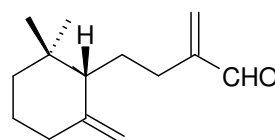
gamma-coronal
